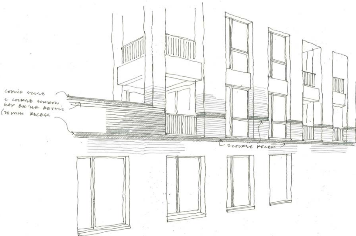
OPTION 2: 2 NO. 20MM RECESSES, 150MM (APPROX) TALL EACH
