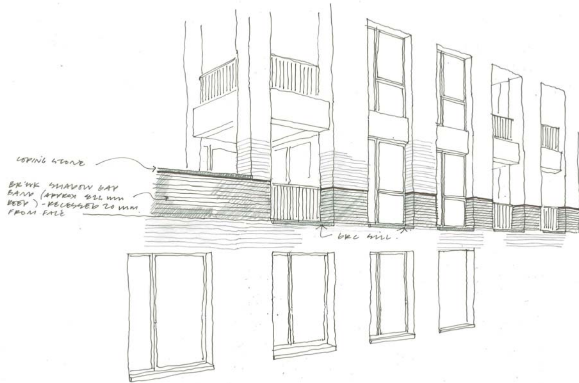
OPTION 1: 20MM RECESS, 825MM (APPROX) TALL
