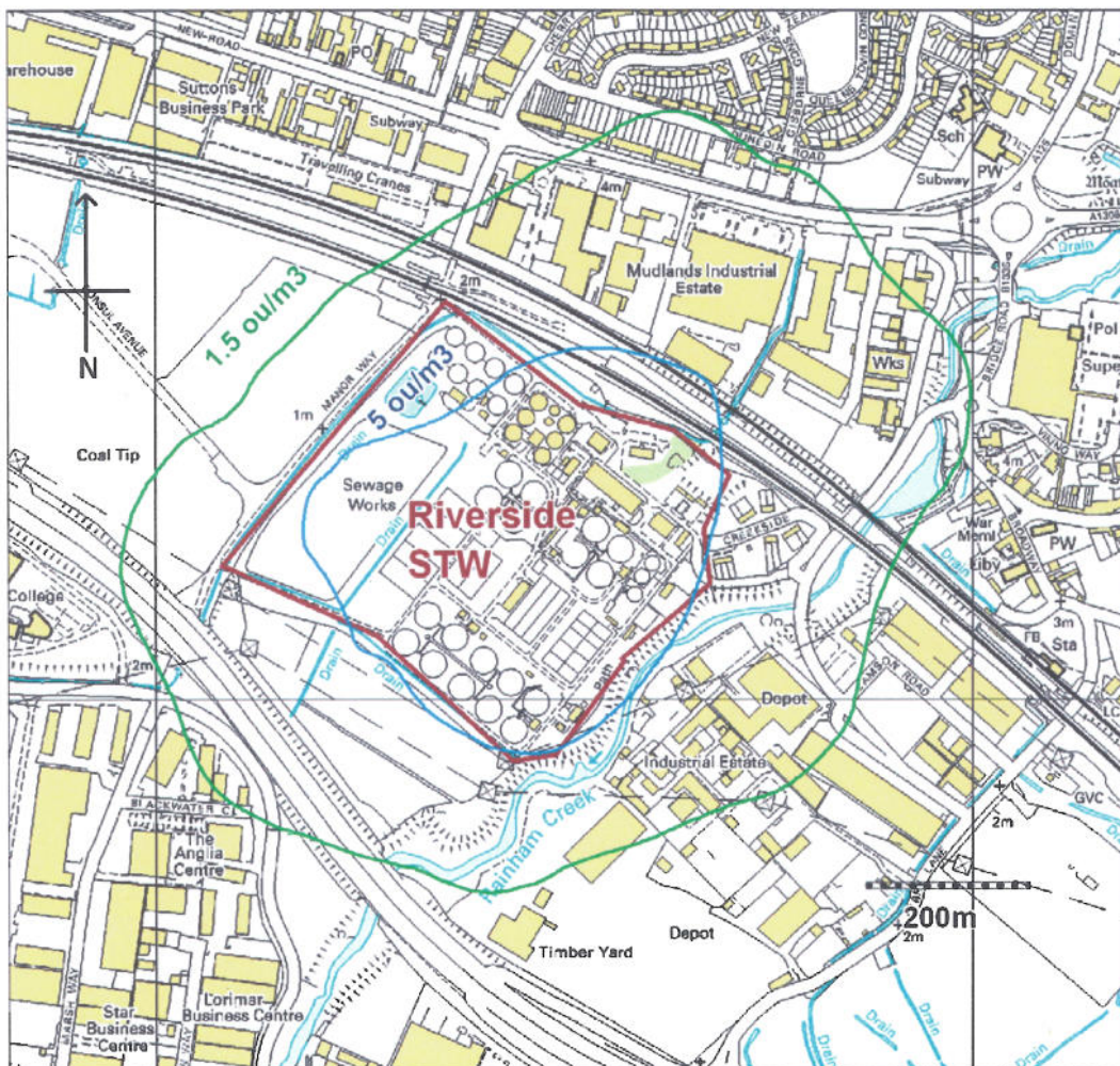
Figure 1: Contours for the revised layout of the extended works
